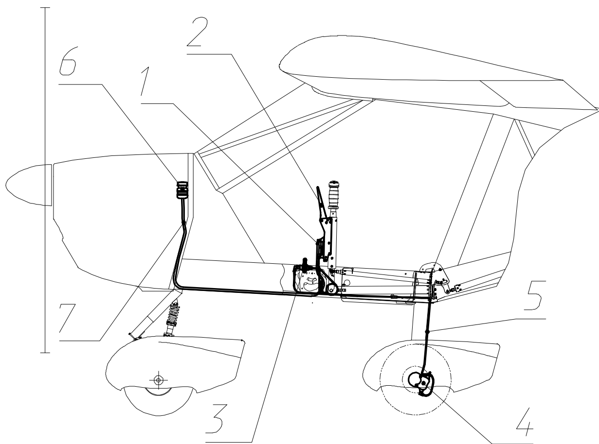
Fig. 8. Brake control system
