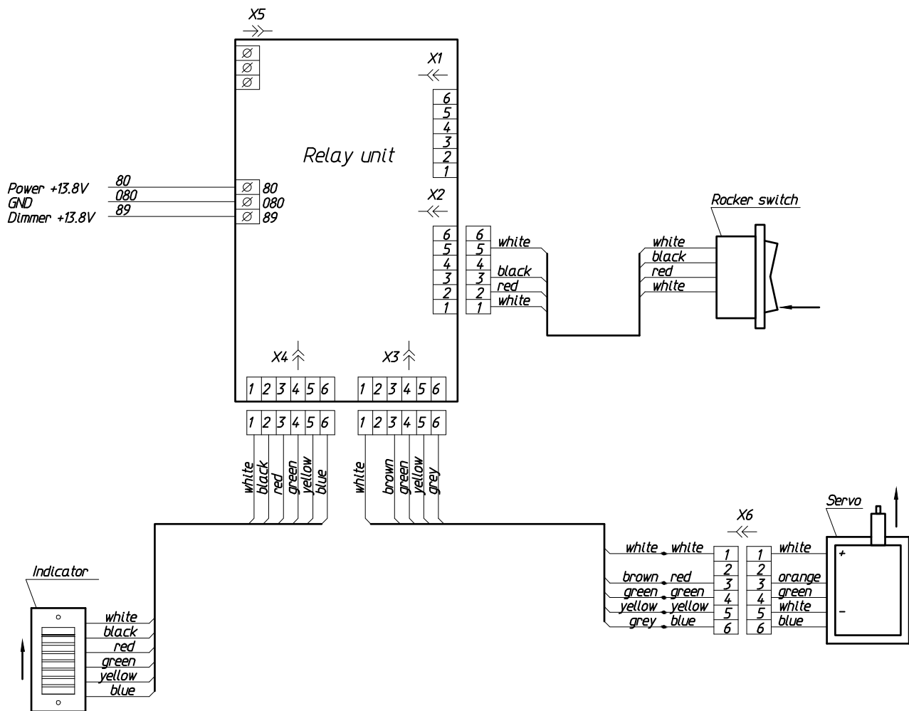
Fig. 16 Wiring diagram of the installation of the Trim. tab control
