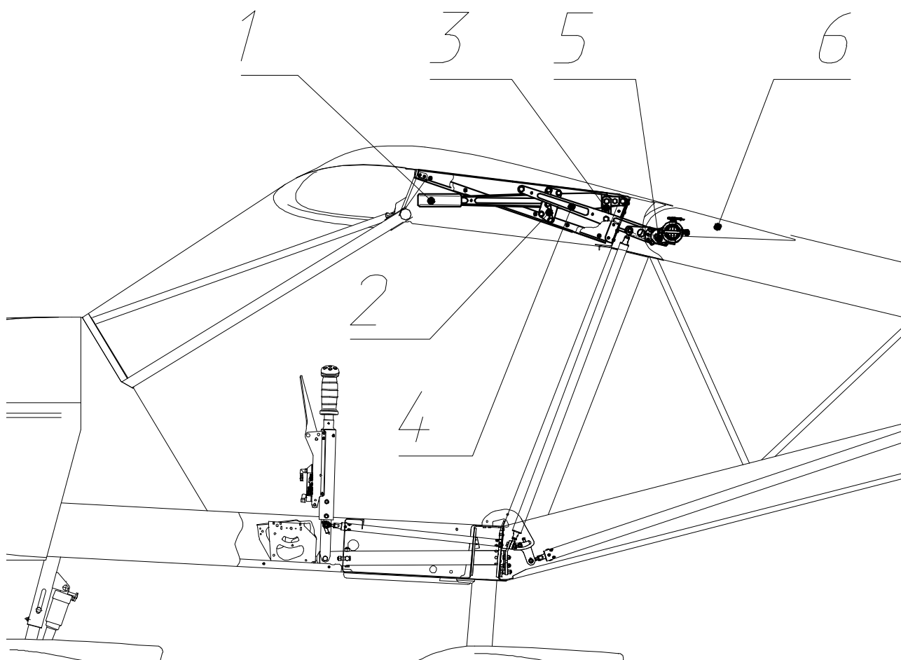
Fig. 7. Flap extension mechanism
