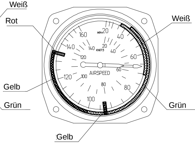
Fahrtmesser [Knoten]
