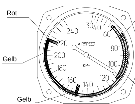
Fahrtmesser [km/h]
